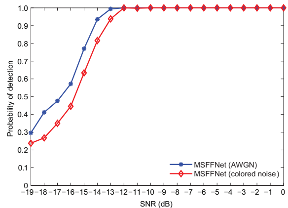
Fig. 13 P_d -SNR curves of the MSFFNet under AWGN and colored noise
