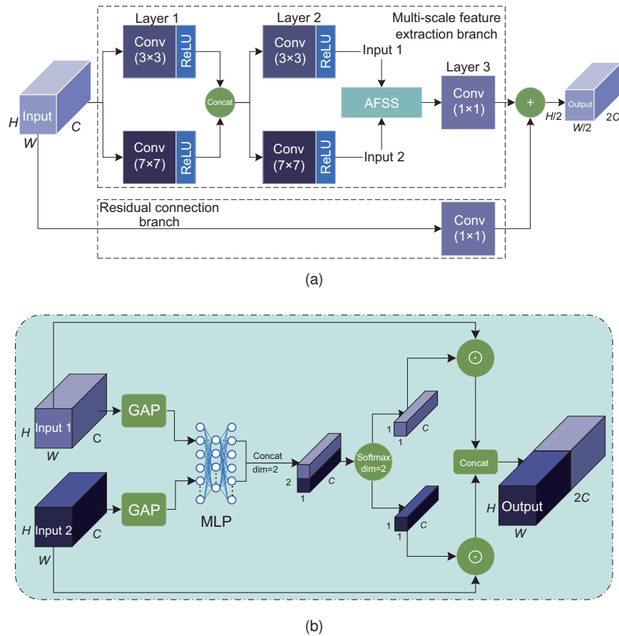
Fig. 4 Illustration of the multi-scale feature extraction (a) and AFSS in the MSFEB (b). \odot : channel-wise multiplication
